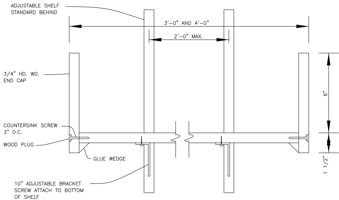
LENGTHWISE SECTION
